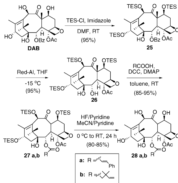
Scheme 9.
