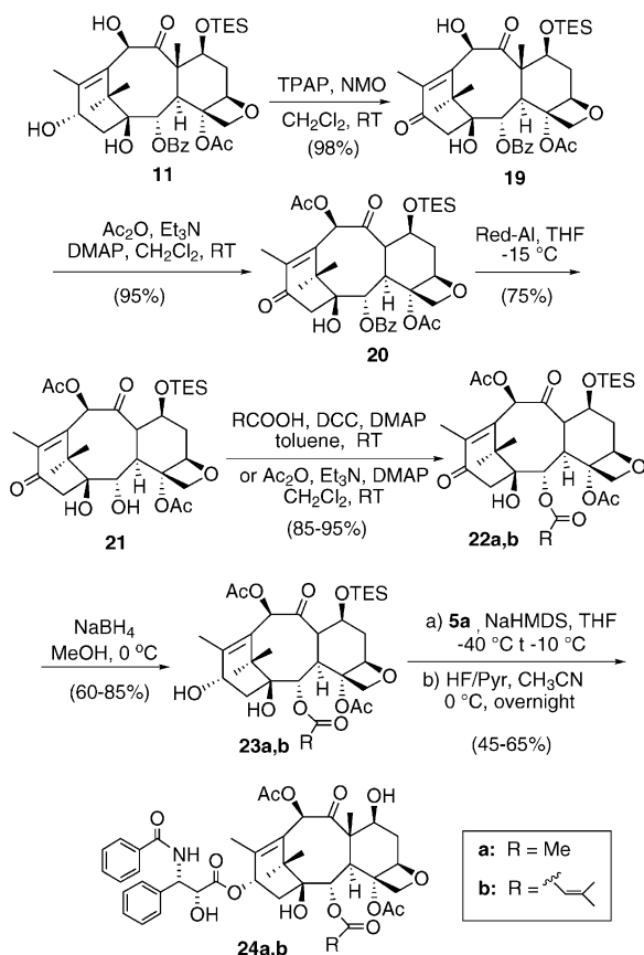
Scheme 8.
