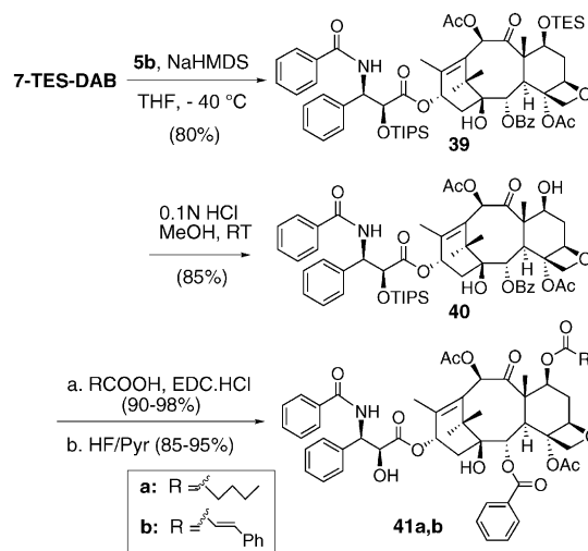
Scheme 13.
