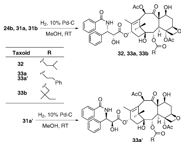
Scheme 11.
